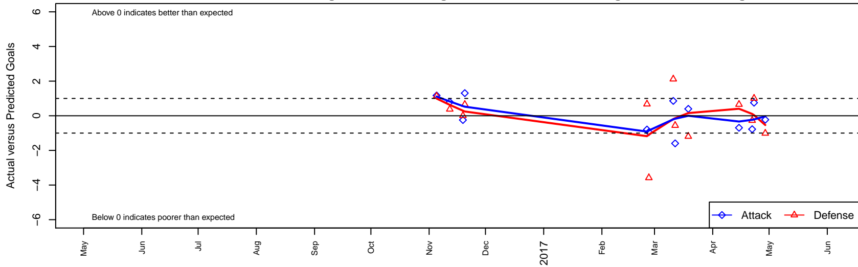
PCU Black 1 B03 Dots are actual minus expected GF (blue circles) and GA (red triangles). Blue line is smoothed change in attack strength. Red is smoothed change in defense strength.
